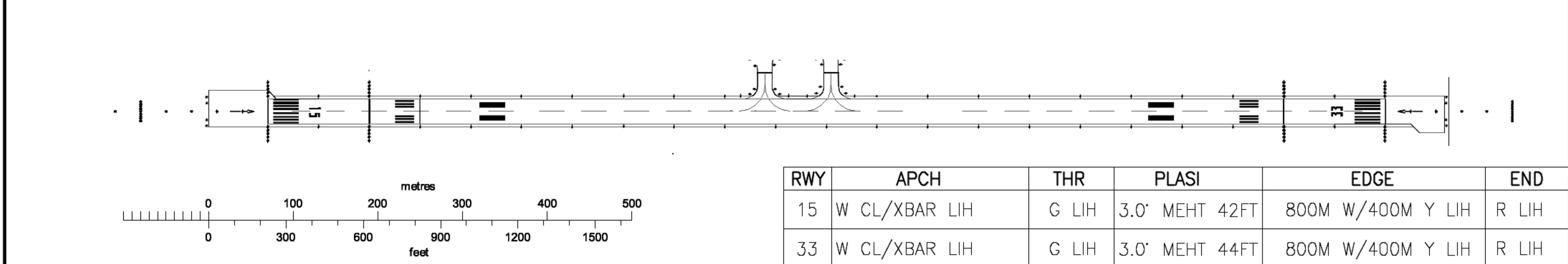
LIGHTING AND MARKING AIDS RWY 15/33 AND EXIT TWY
