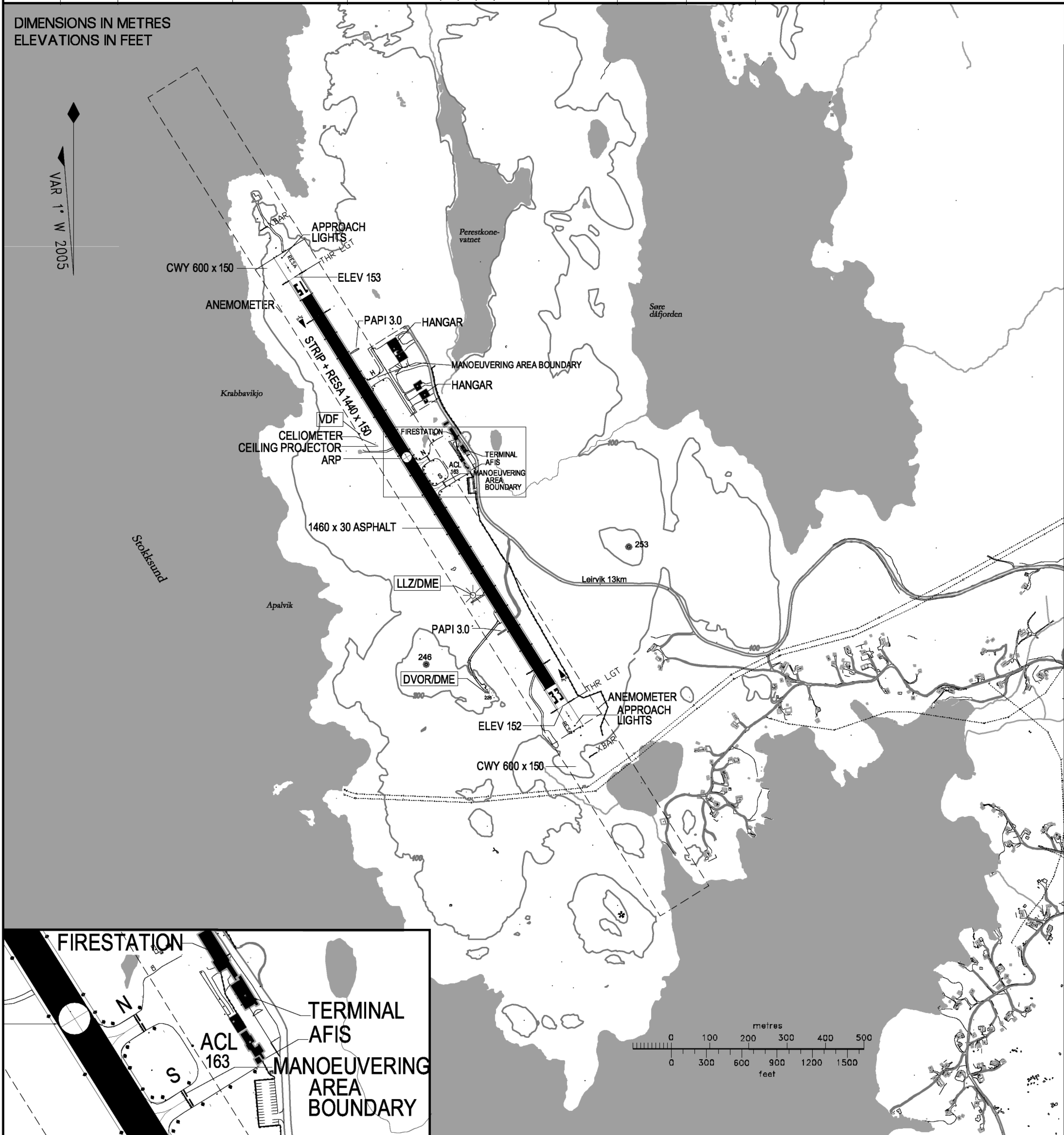
LIGHTING AND MARKING AIDS RWY 15/33 AND EXIT TWY
